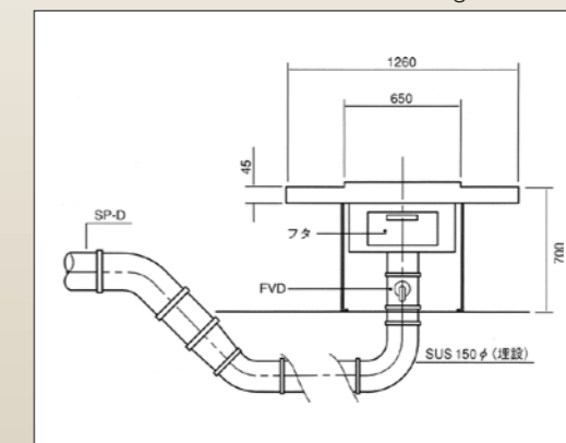
●基本施工図 Installation Drawing
